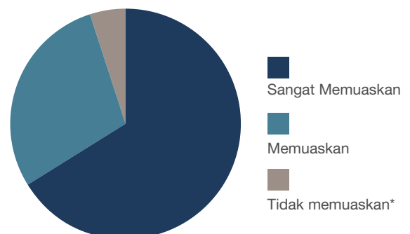
SMS Rating
