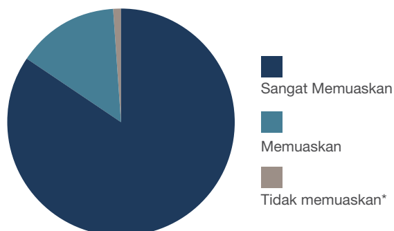
Mesin Rating
